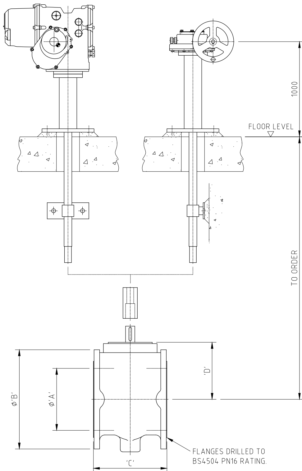
VALVE DIMENSION TABLE
